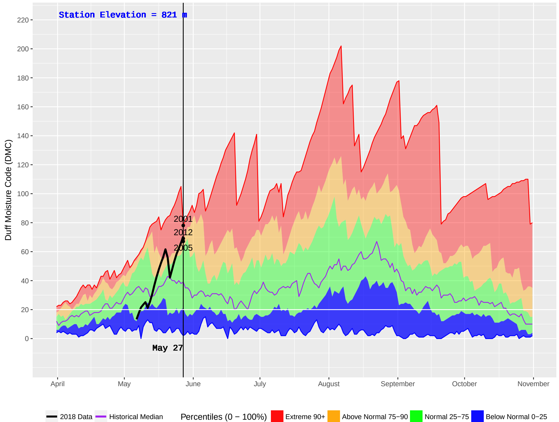
KNIFE (225) : Historical (1991–2016) and Current (2018) Noon Duff Moisture Code (DMC)
