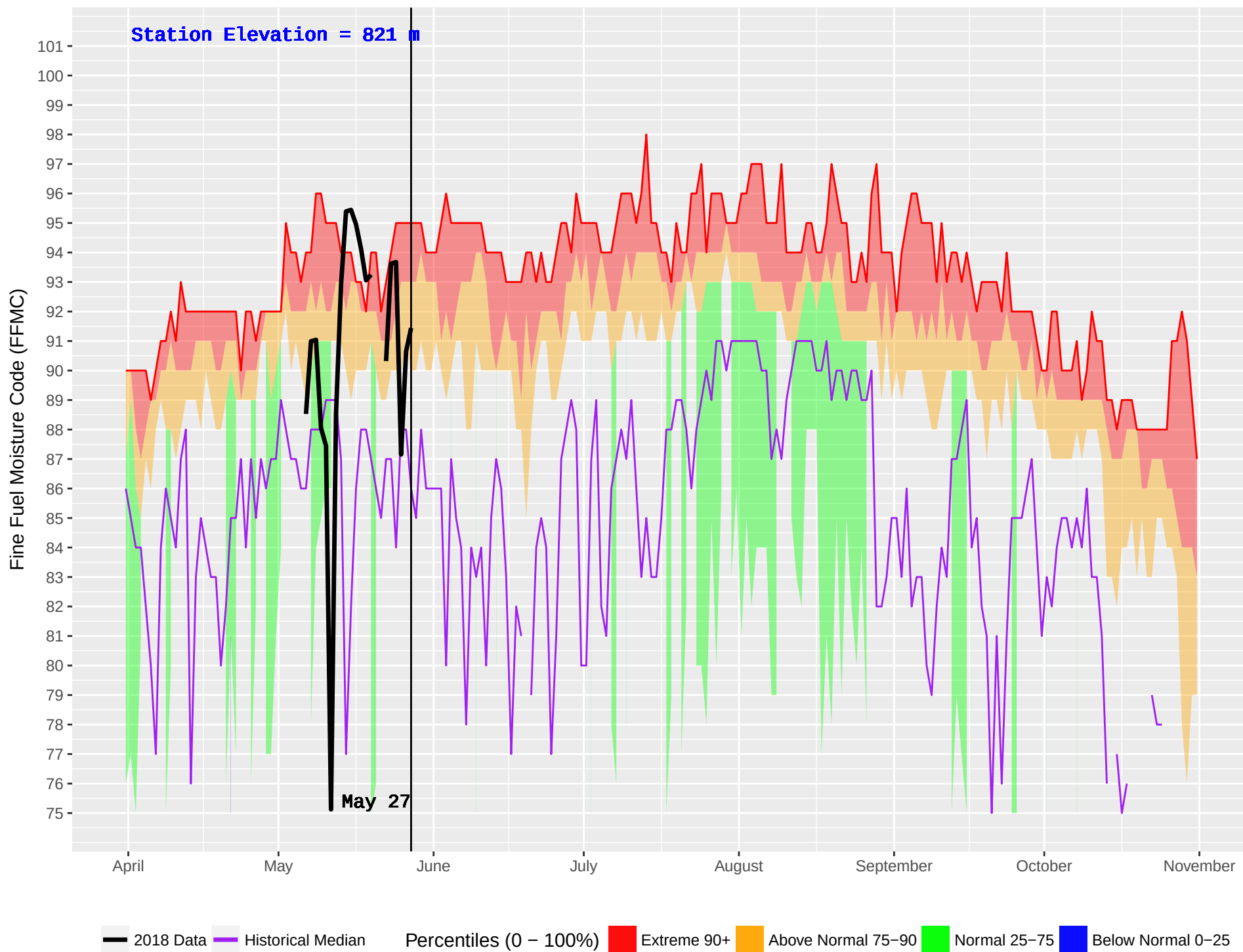
KNIFE (225) : Historical (1991–2016) and Current (2018) Noon Fine Fuel Moisture Code (FFMC)
